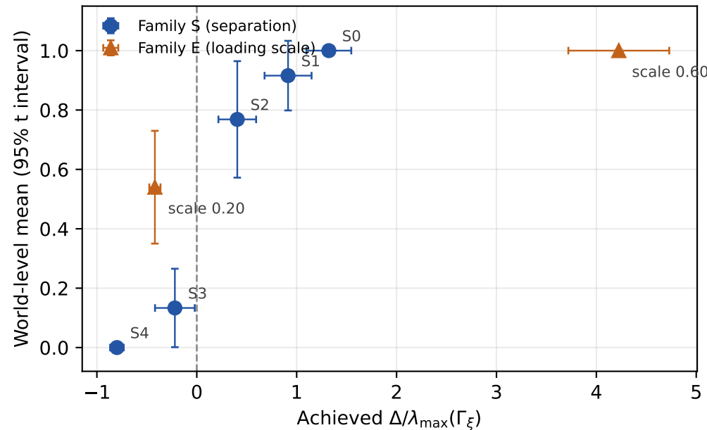
True r is a fixed point
