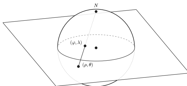
Figure 2.3: For each point on the sphere (except for its north pole) a line is drawn from the north pole through the point and extending to the equatorial plane. The corresponding point on the plane is where the line intersects the plane. The rectangular coordinates of this point on the plane are the Riemann coordinates of the point on the sphere. The points on the plane can also be specified with polar coordinates (\rho, \theta) and the points on the sphere are specified both by Riemann coordinates and the traditional colatitude and longitude (\varphi, \lambda) .
