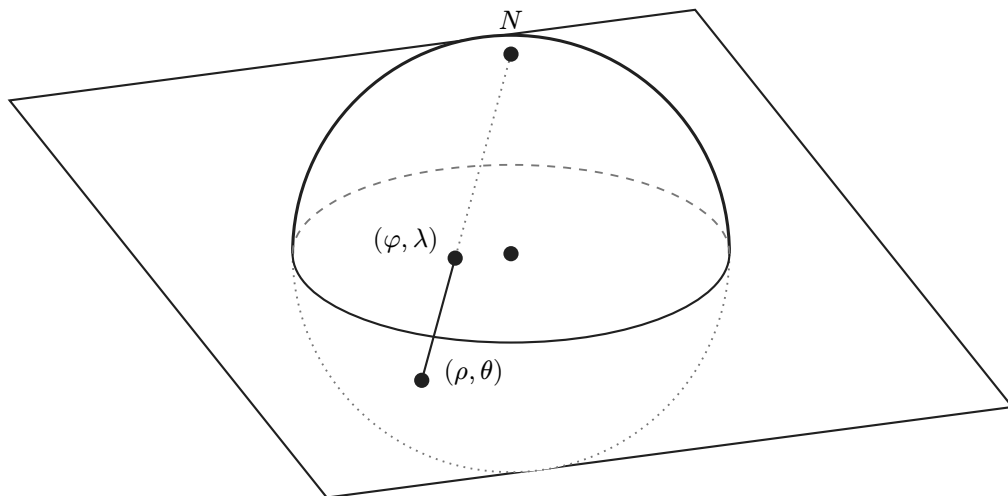
Figure 2.3: Riemann coordinates on the sphere
