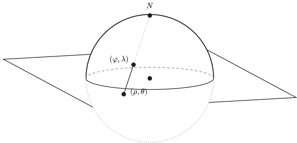
Figure 2.3: Riemann coordinates on the sphere
