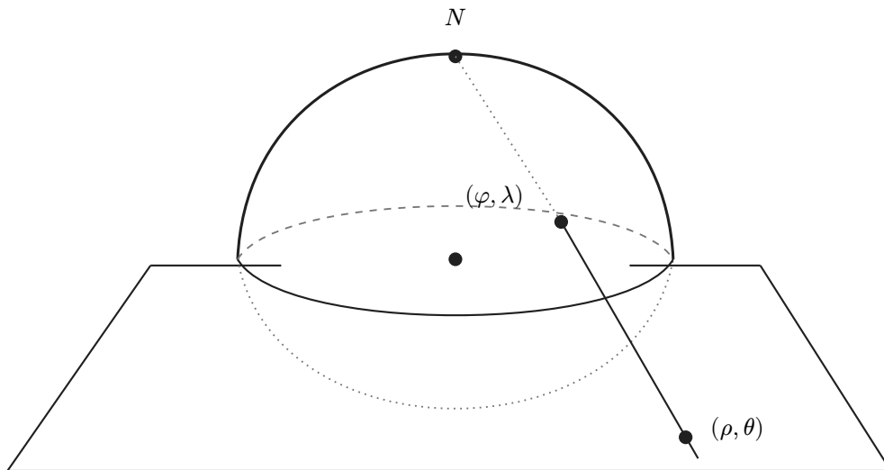
Figure 2.3: Riemann coordinates on the sphere
