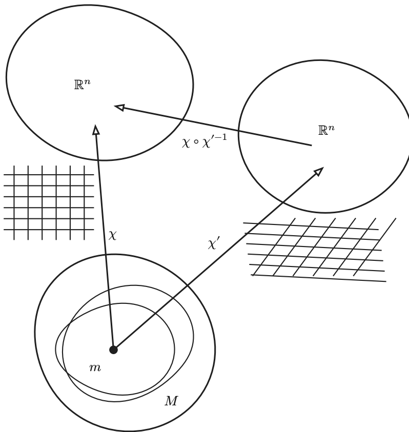
Figure 2.1: Overlapping coordinate patches
