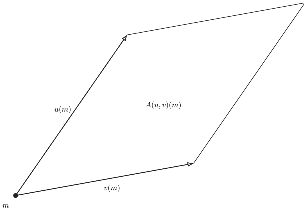
Figure 5.1: Oriented area
