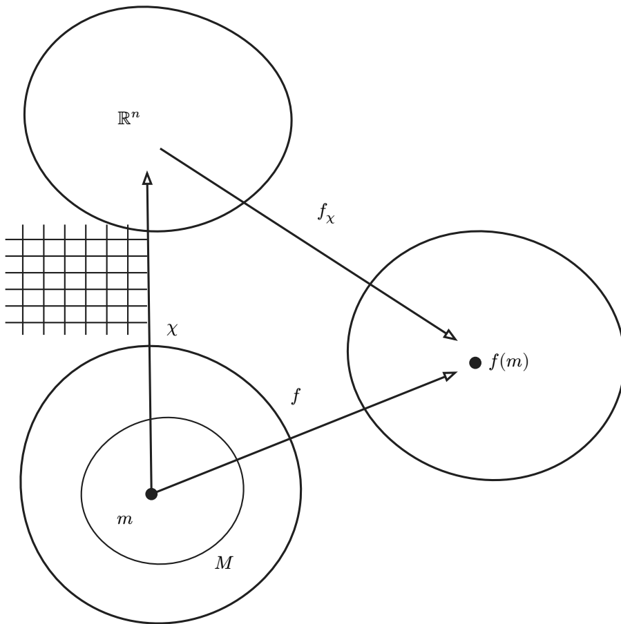
Figure 2.2: A manifold function in coordinates
