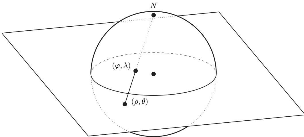
Figure 2.3: Riemann coordinates on the sphere
