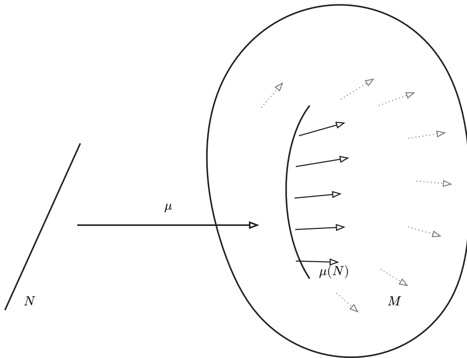
Figure 6.1: A vector field over a map
