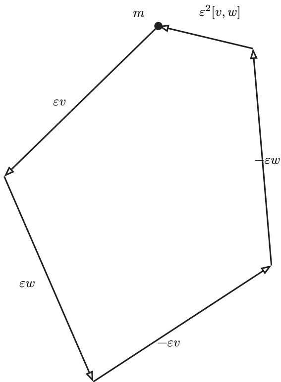
Figure 4.2: The commutator loop
