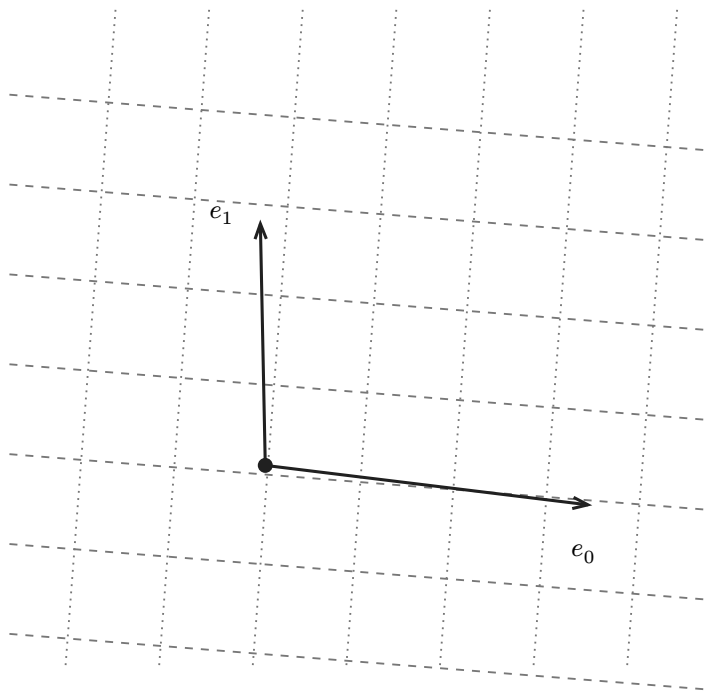
Figure 4.1: A basis and its dual foliations
