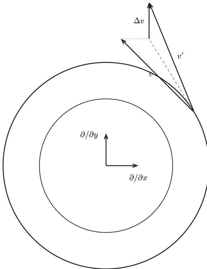
Figure 7.1: Parallel transport in a circular field
