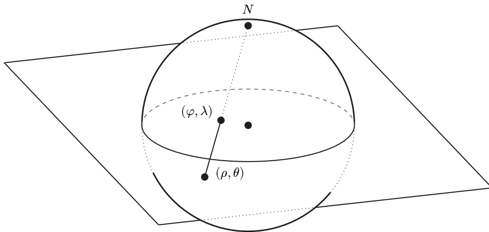
Figure 2.3: Riemann coordinates on the sphere
