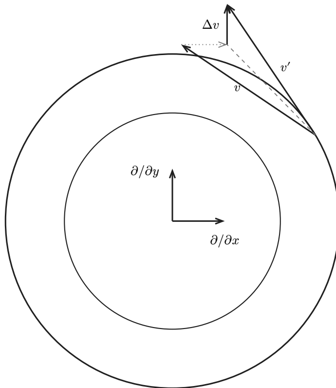
Figure 7.1: Parallel transport in a circular field
