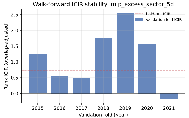
Figure 4: Walk-forward per-fold ICIR for the headline run.
