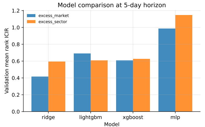
Figure 4: Validation mean rank ICIR by model at the 5-day horizon.
