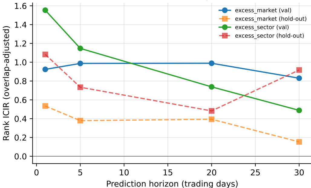
Best-model rank ICIR by horizon
