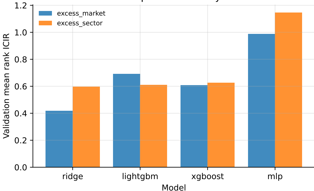
Model comparison at 5-day horizon
