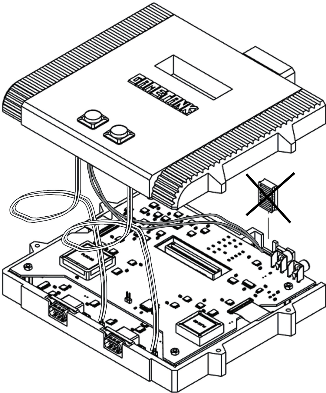
Figure 23: Wires from buttons plug into headers on board. Ignore vent piece in diagram.
