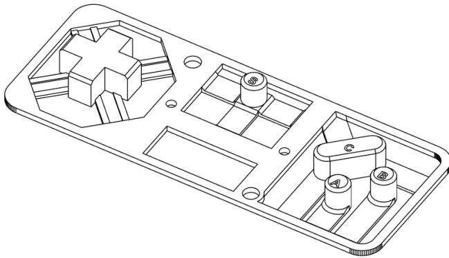
Figure 8: Button Flexure, Multi Material Print Labels (Provided separately)
