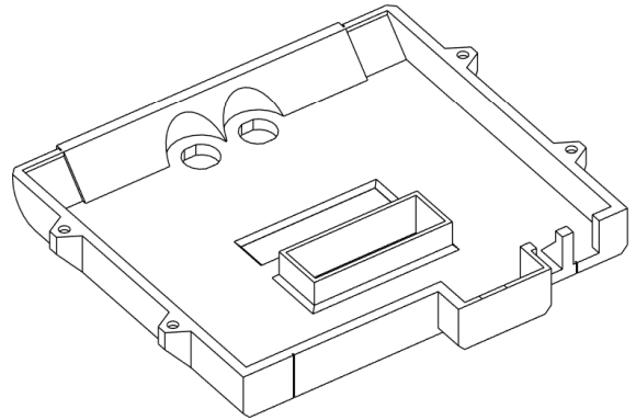
Figure 2: Upper Enclosure Body (Underside view)
