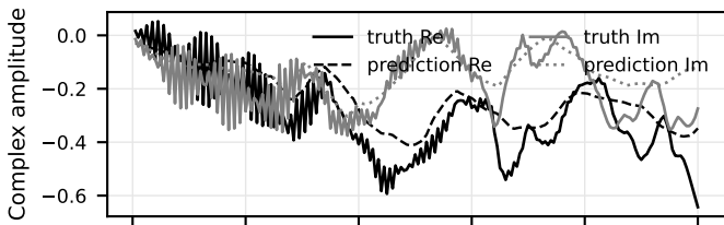
(c) Crosstalk S_{8,1}
