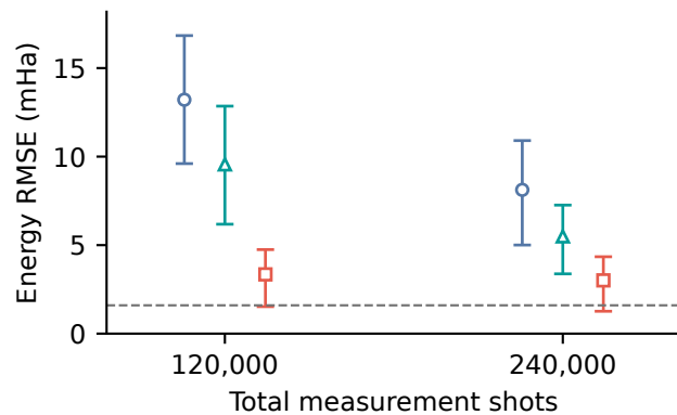
b N 2 , MC-PDFT
