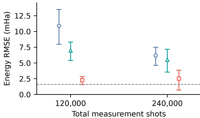
d CO, MC-PDFT
