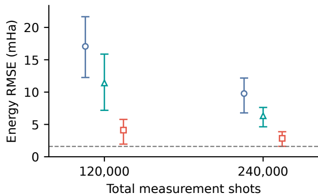
a N 2 , Hamiltonian
