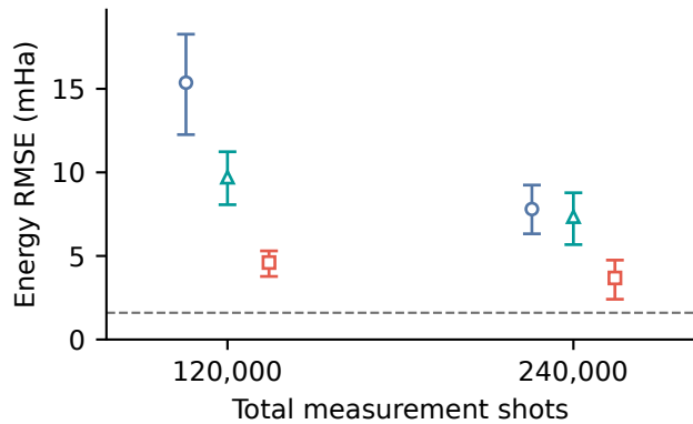
c CO, Hamiltonian
