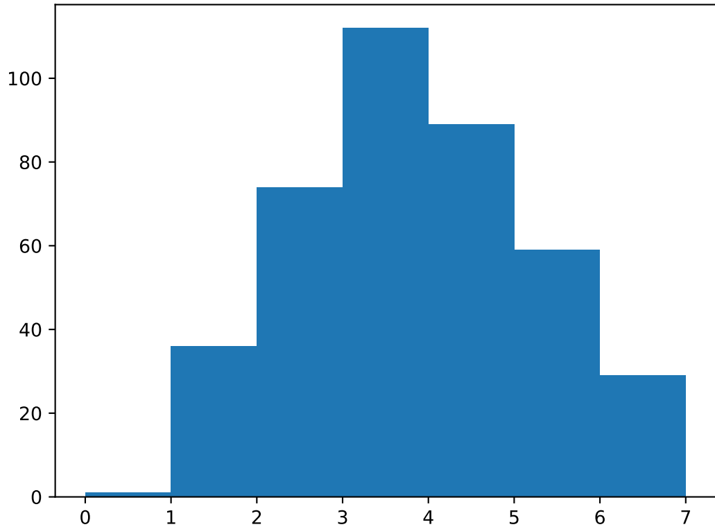
Distribution of shortest-path lengths from starting node
