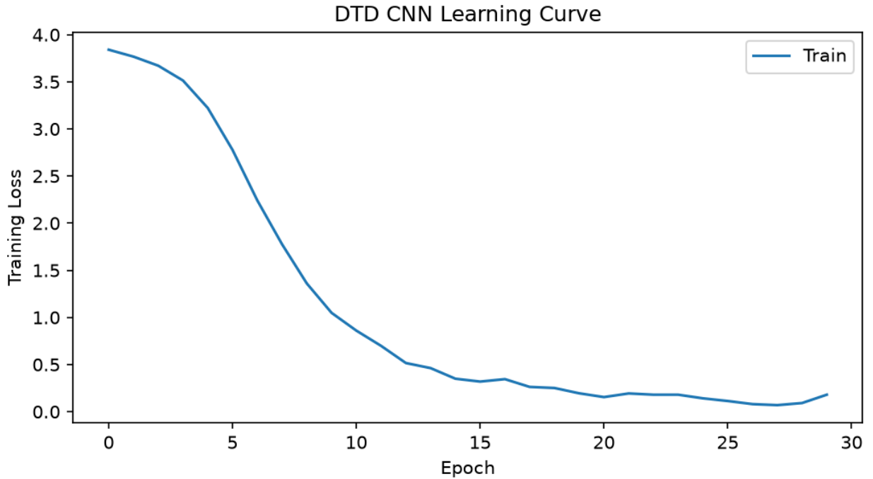
Figure 5: DTD lightweight-CNN training loss over the full 30-epoch schedule. Loss falls below 0.2 with no plateau, while held-out test accuracy worsens relative to a 10-epoch run (11.52%→8.51%) – a classic overfitting signature on a dataset with only \sim 96 training images per class and no augmentation.
