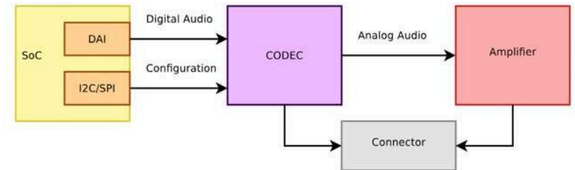
Example of an embedded system sound card
