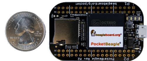
PocketBeagle
