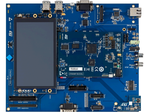
STM32MP157C-EV1 eval board
