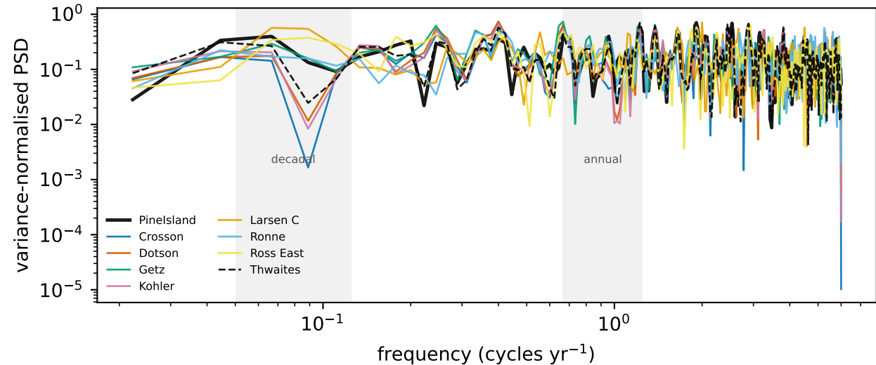
Spectral shape of basin-integrated SMB residual (flat = white)
