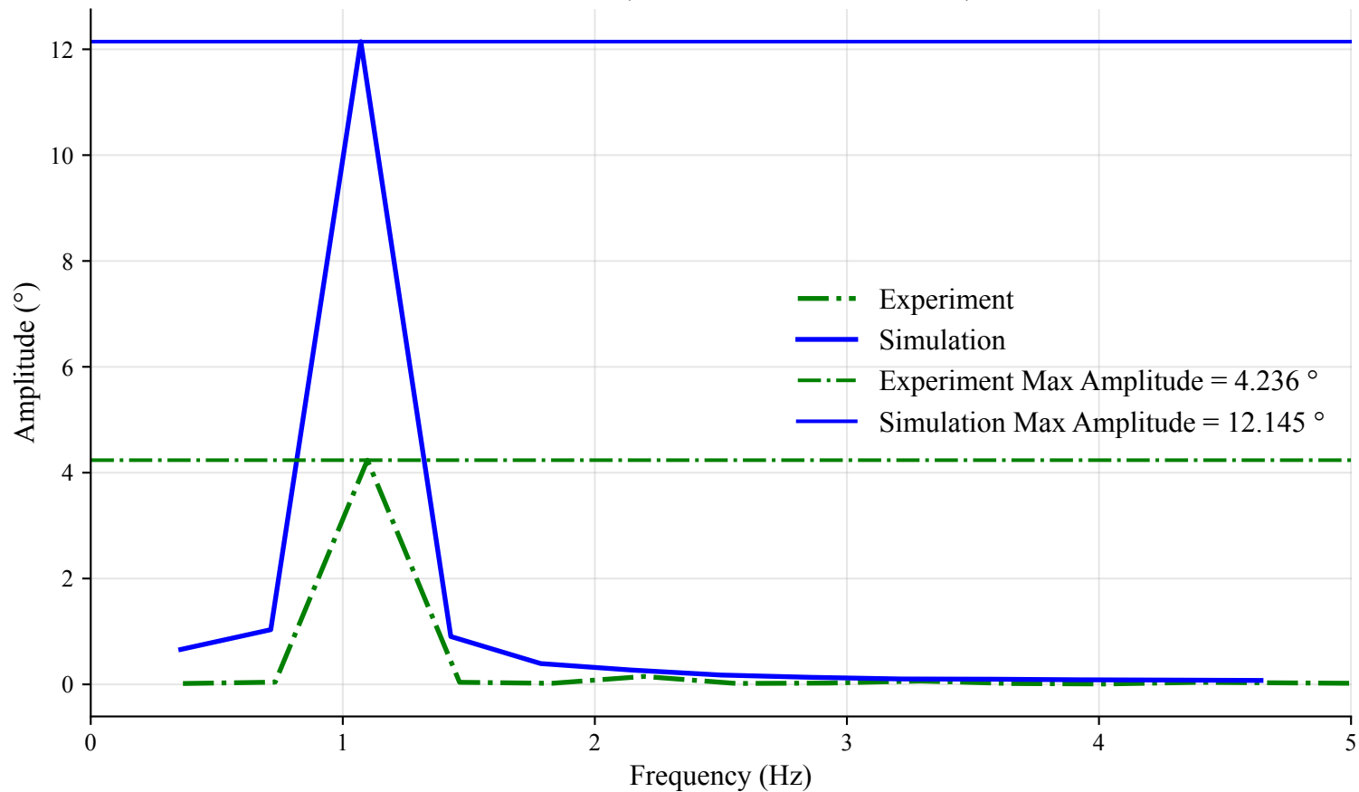
FFT of Pitch (Time Window: 18s to 20.73s)
