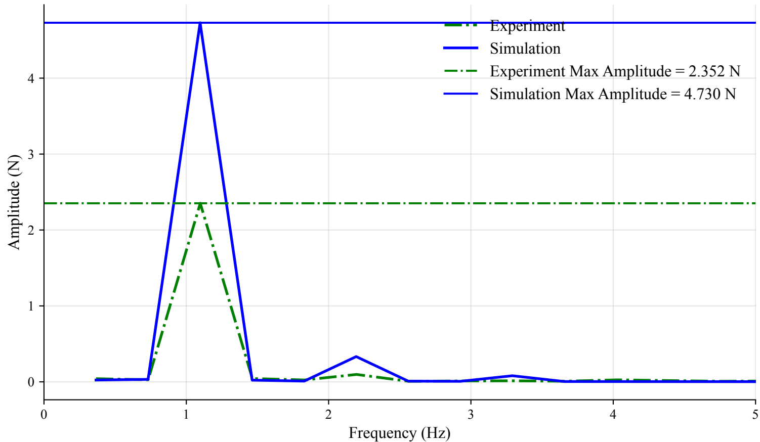
FFT of Front Tension (Time Window: 18s to 20.73s)
