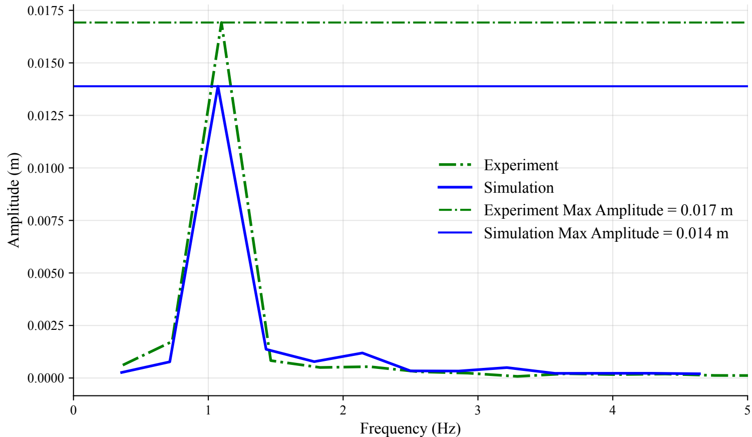
FFT of Heave (Time Window: 18s to 20.73s)
