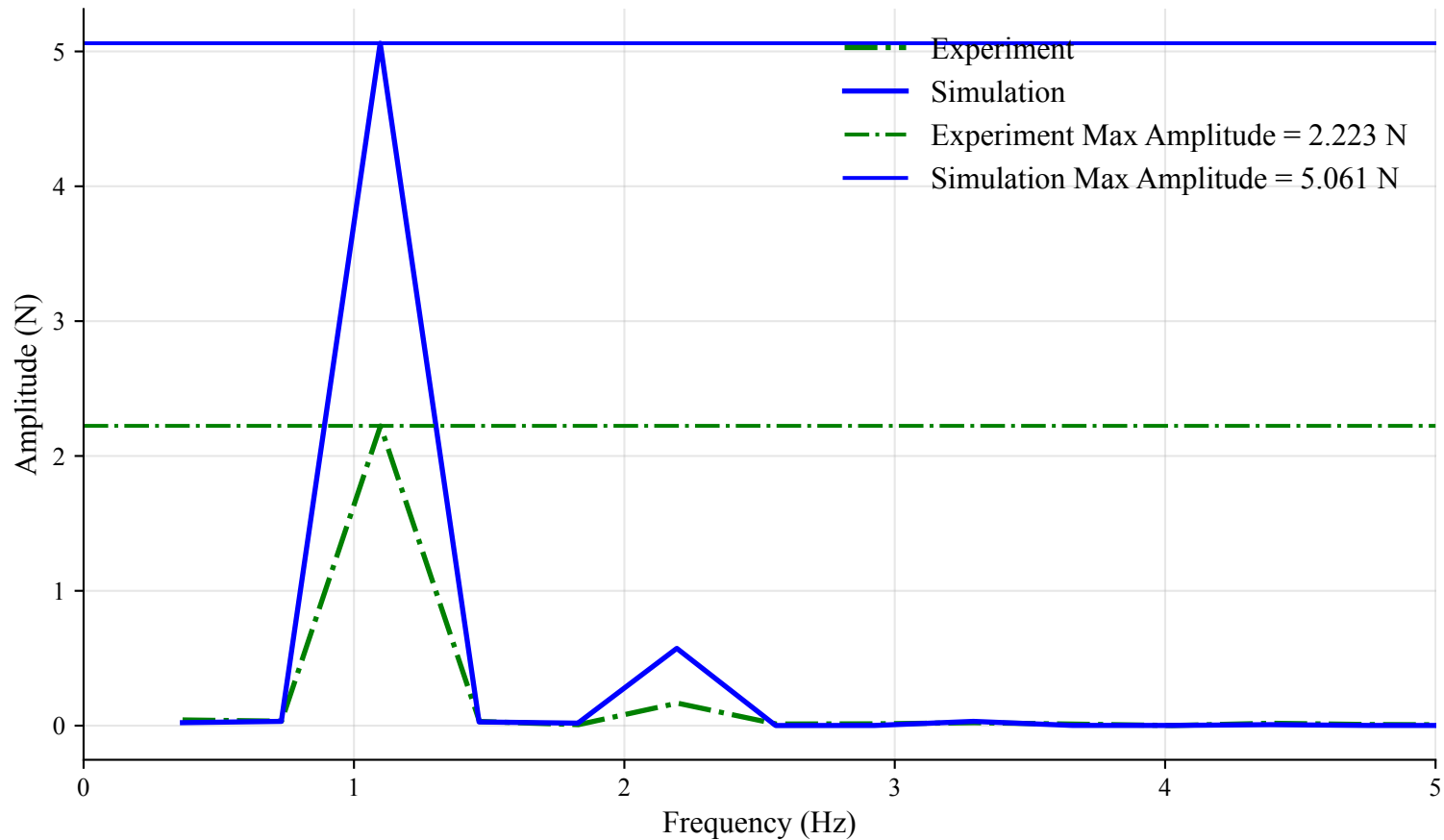
FFT of Rear Tension (Time Window: 18s to 20.73s)
