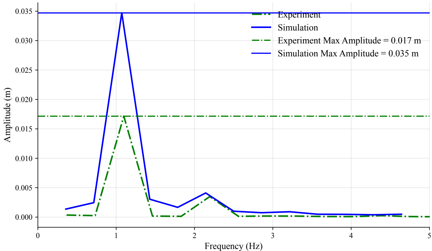
FFT of Surge (Time Window: 18s to 20.73s)
