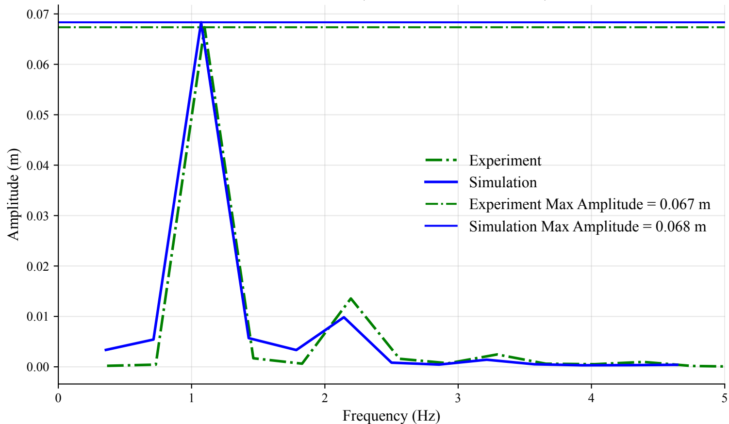
FFT of Wave Probe (Time Window: 18s to 20.73s)
