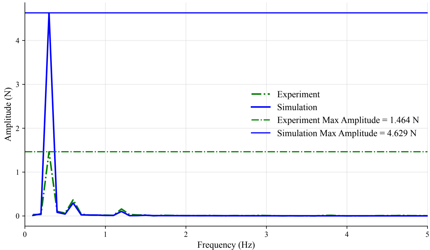
FFT of Rear Tension (Time Window: 18s to 27.99s)
