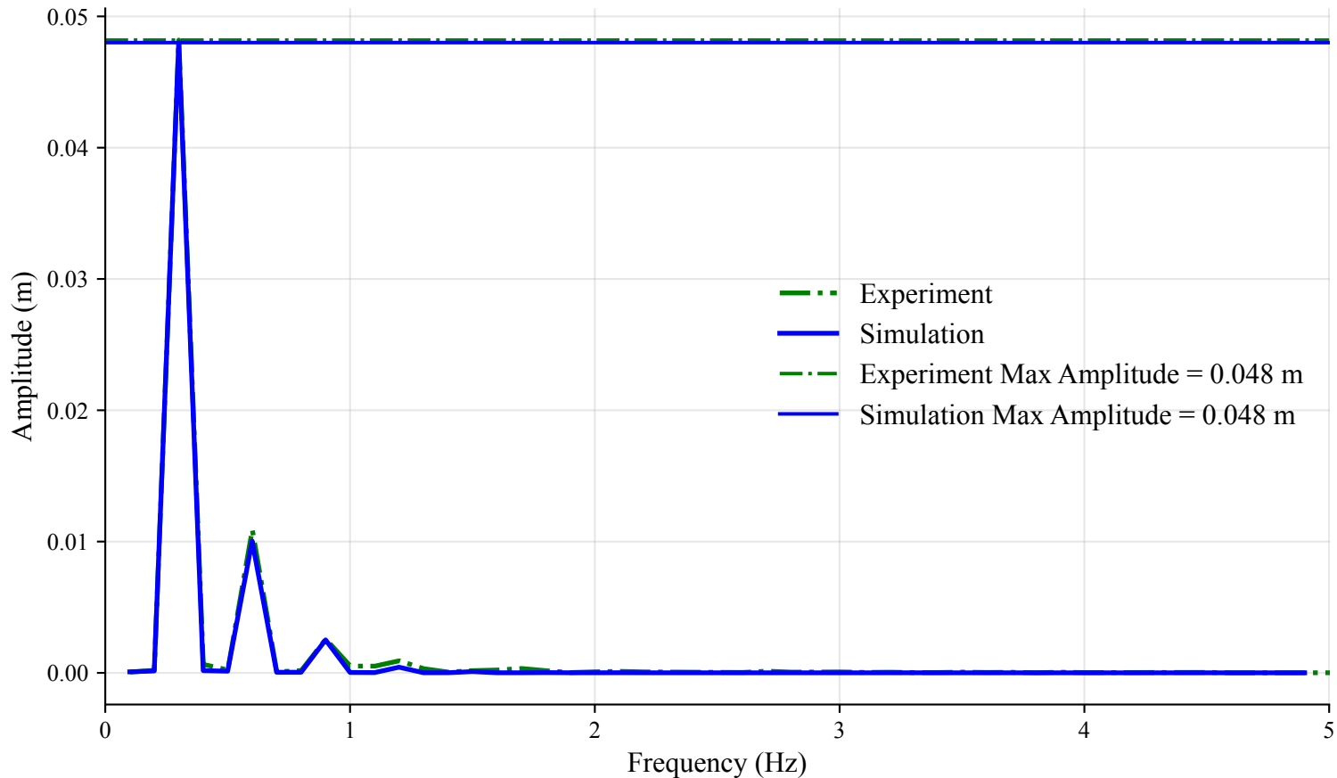
FFT of Wave Probe (Time Window: 18s to 27.99s)
