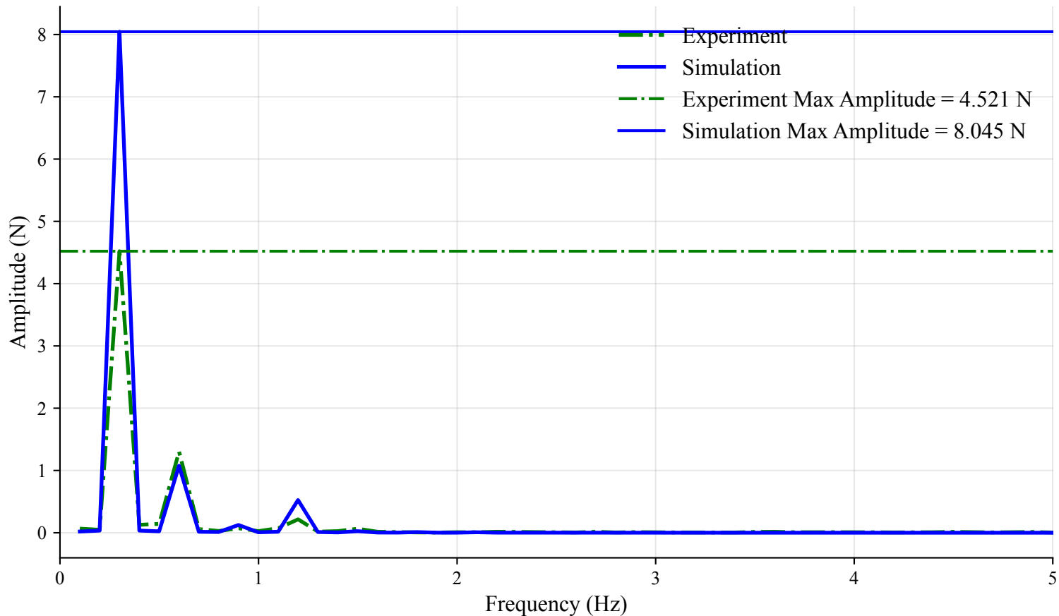
FFT of Front Tension (Time Window: 18s to 27.99s)
