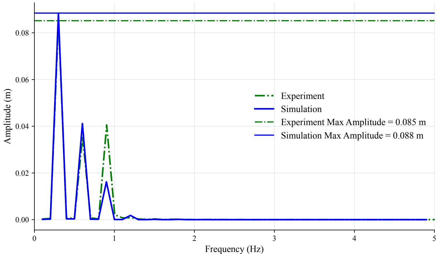
FFT of Heave (Time Window: 18s to 27.99s)
