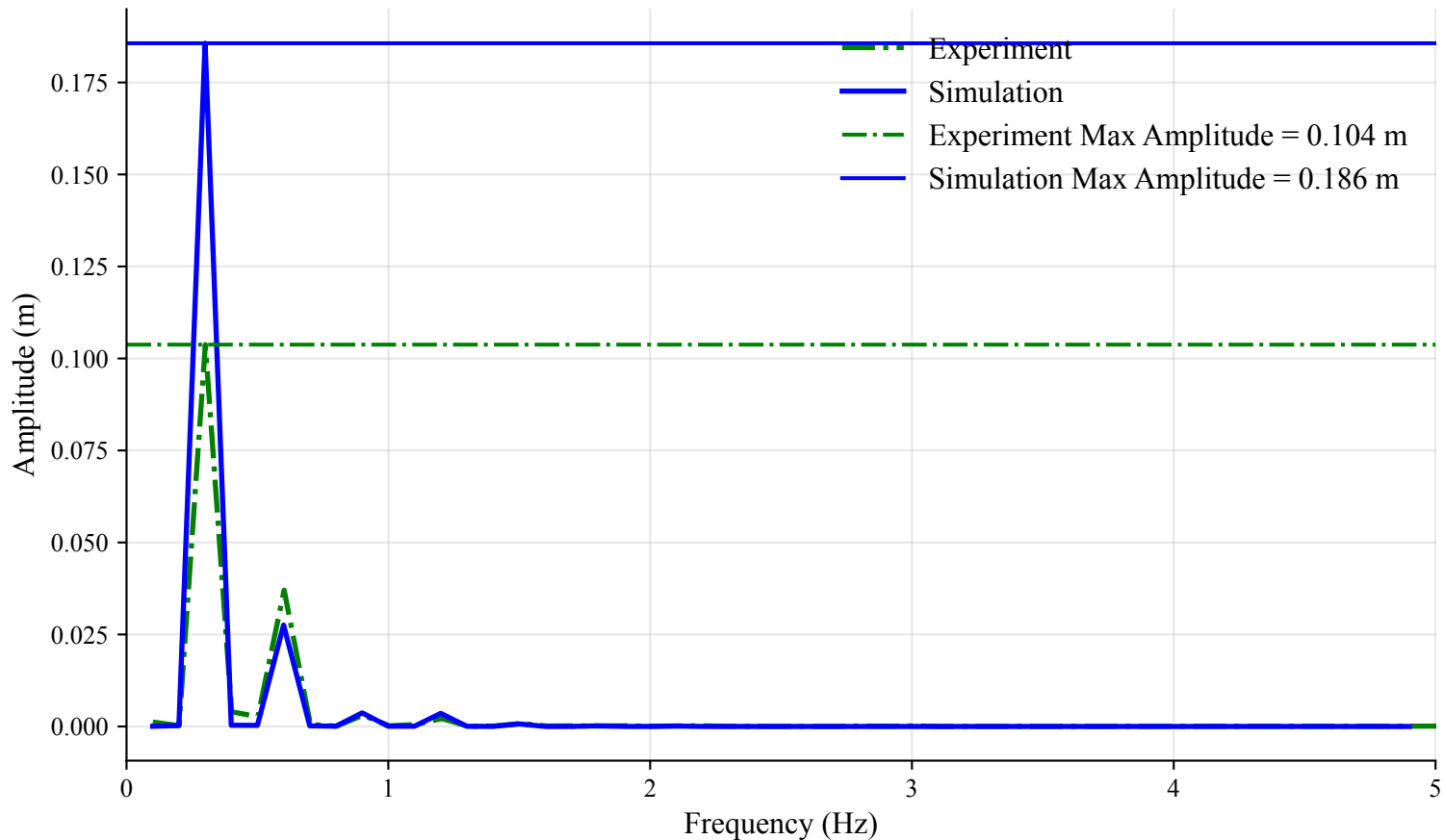
FFT of Surge (Time Window: 18s to 27.99s)
