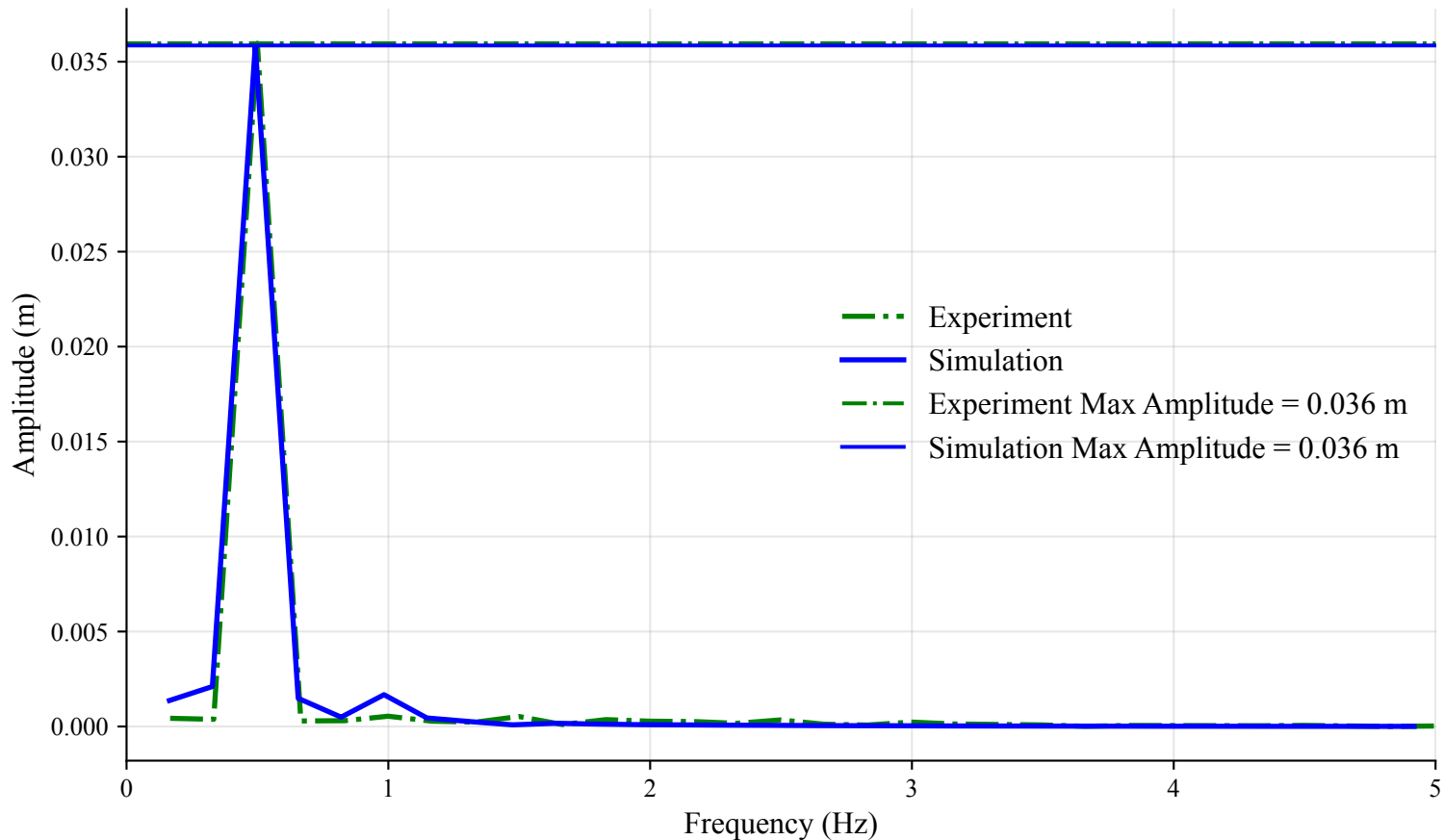
FFT of Wave Probe (Time Window: 18s to 24s)
