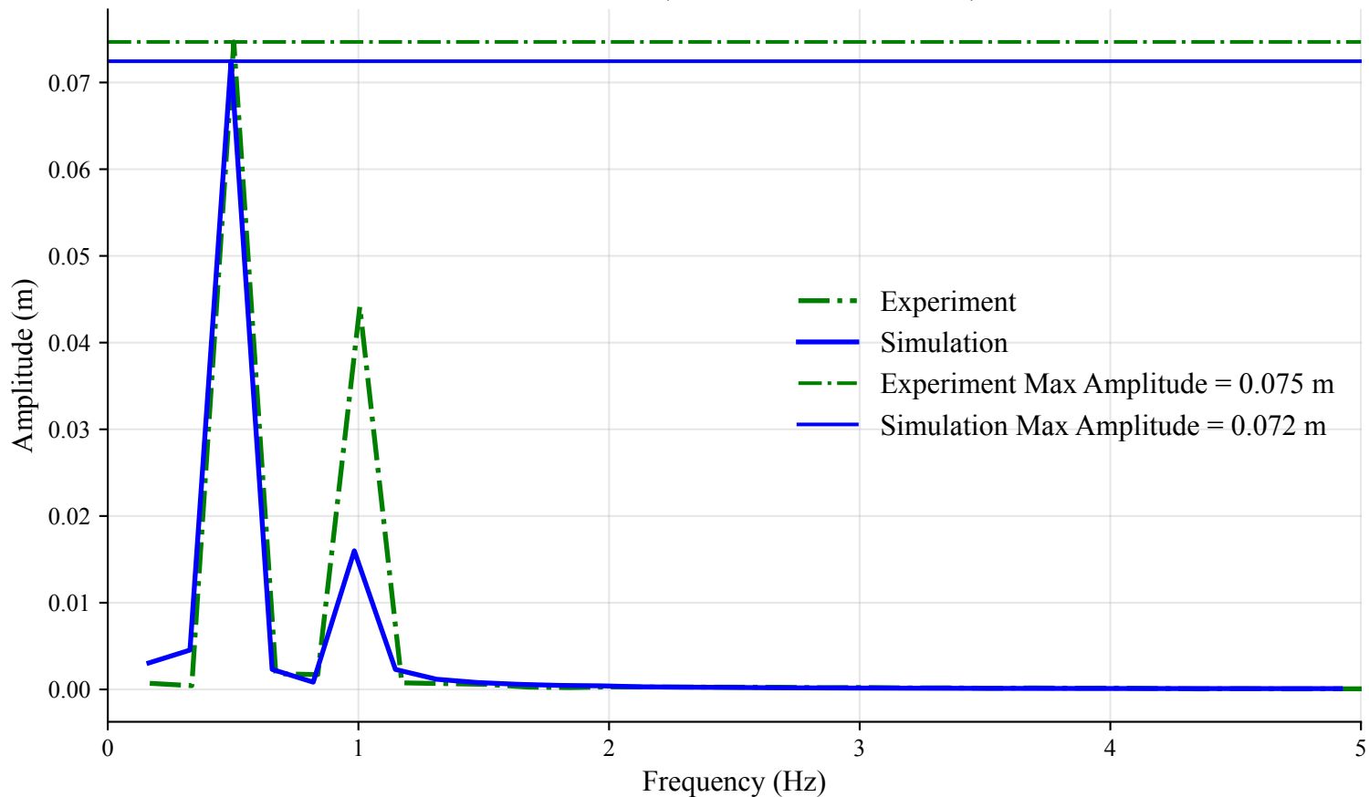
FFT of Heave (Time Window: 18s to 24s)
