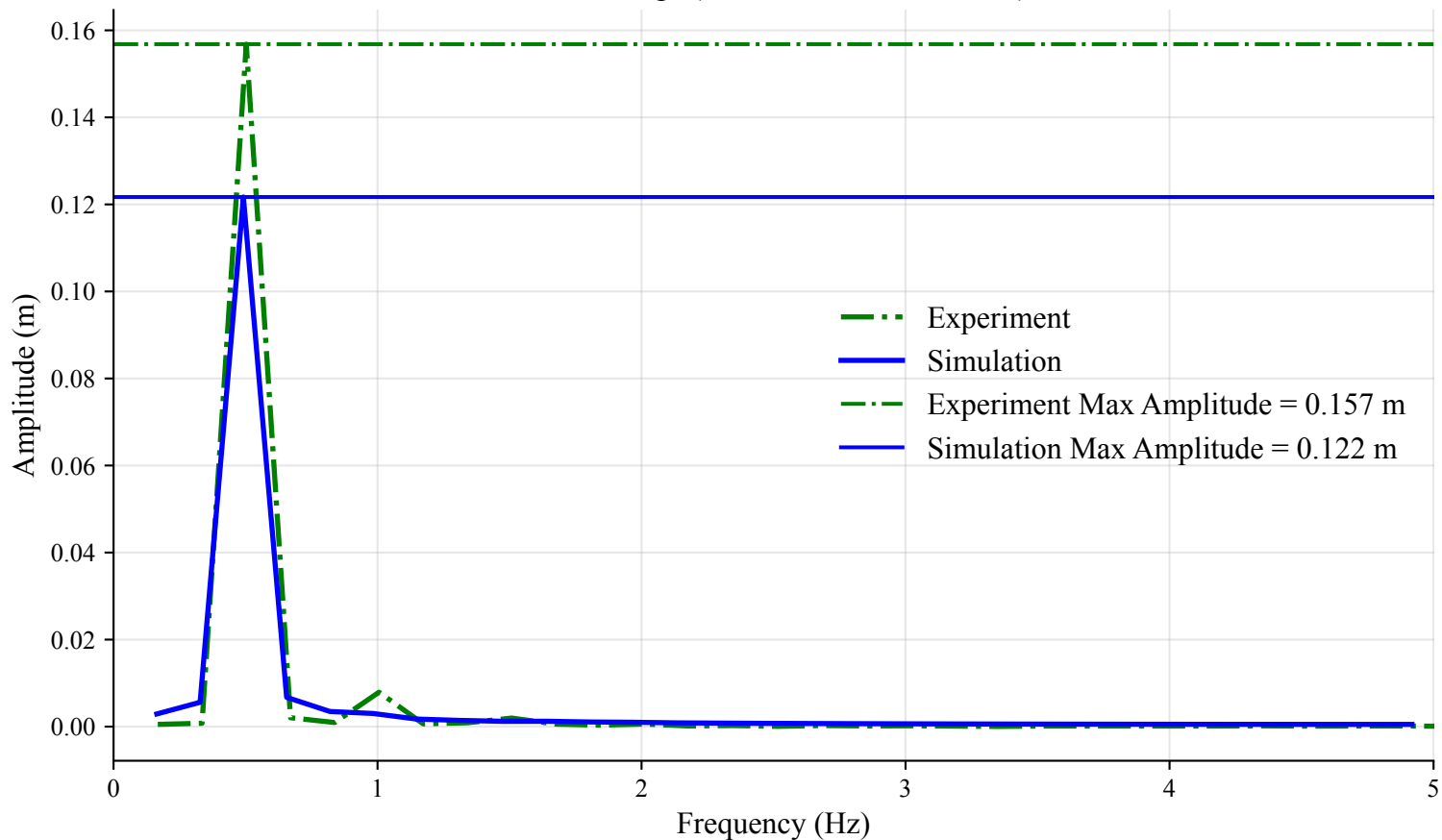
FFT of Surge (Time Window: 18s to 24s)
