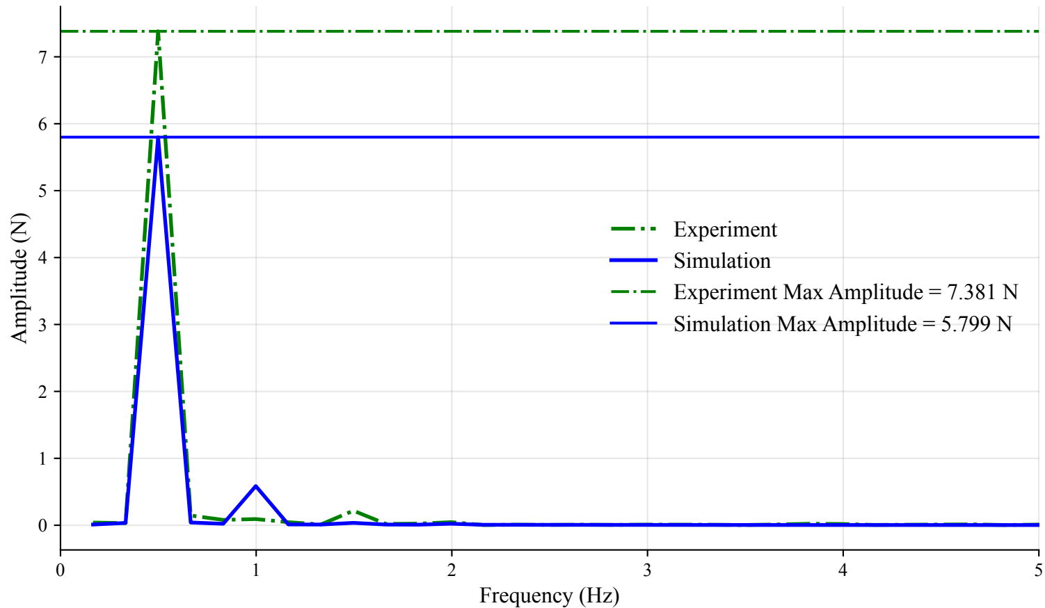
FFT of Rear Tension (Time Window: 18s to 24s)
