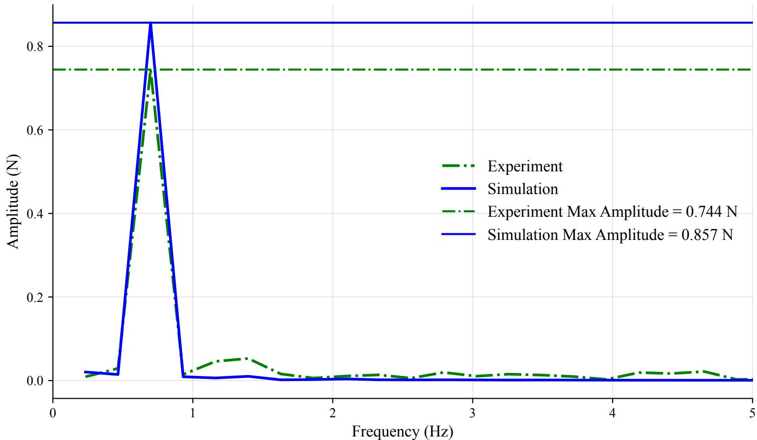
FFT of Front Tension (Time Window: 18s to 22.29s)
