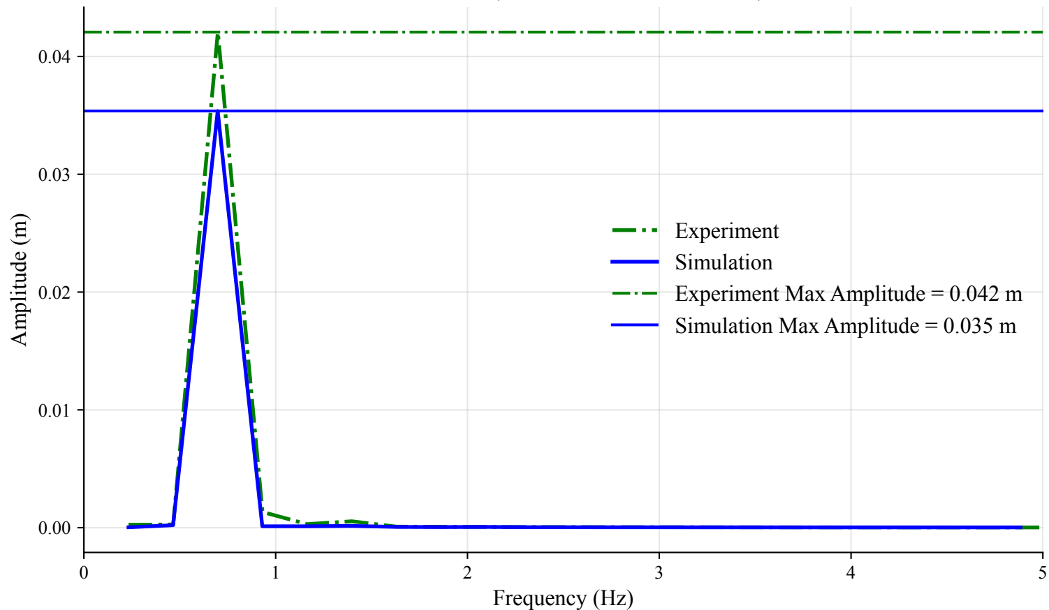
FFT of Heave (Time Window: 18s to 22.29s)
