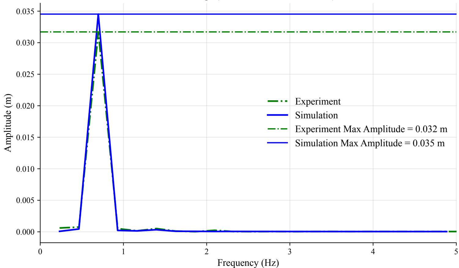
FFT of Surge (Time Window: 18s to 22.29s)
