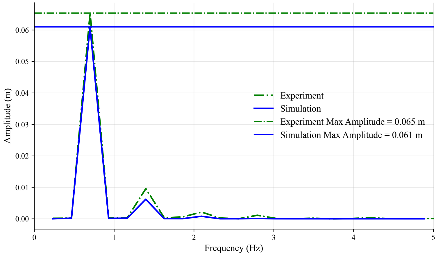
FFT of Wave Probe (Time Window: 18s to 22.29s)
