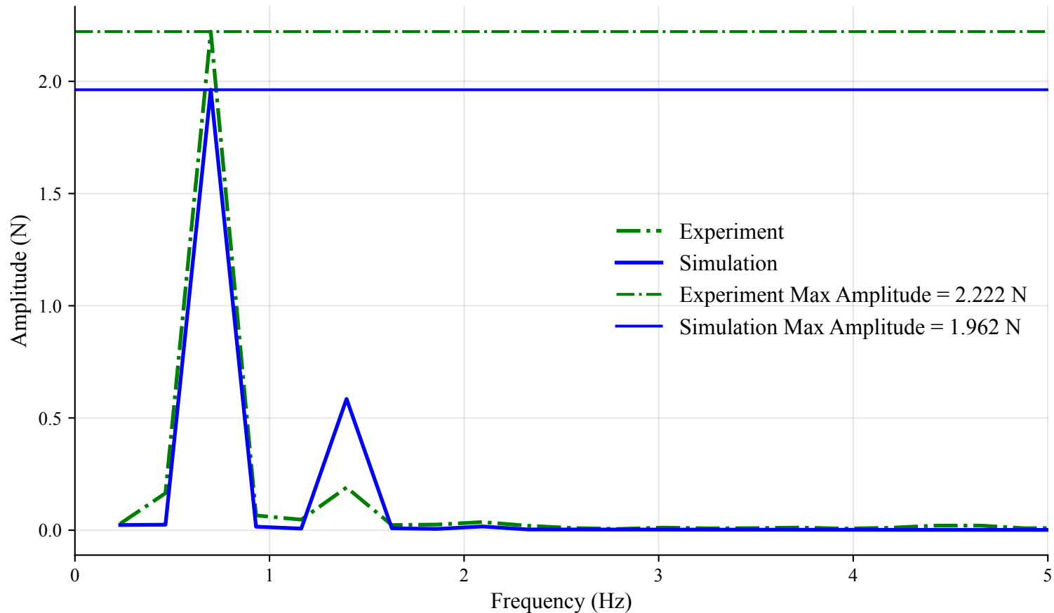
FFT of Rear Tension (Time Window: 18s to 22.29s)
