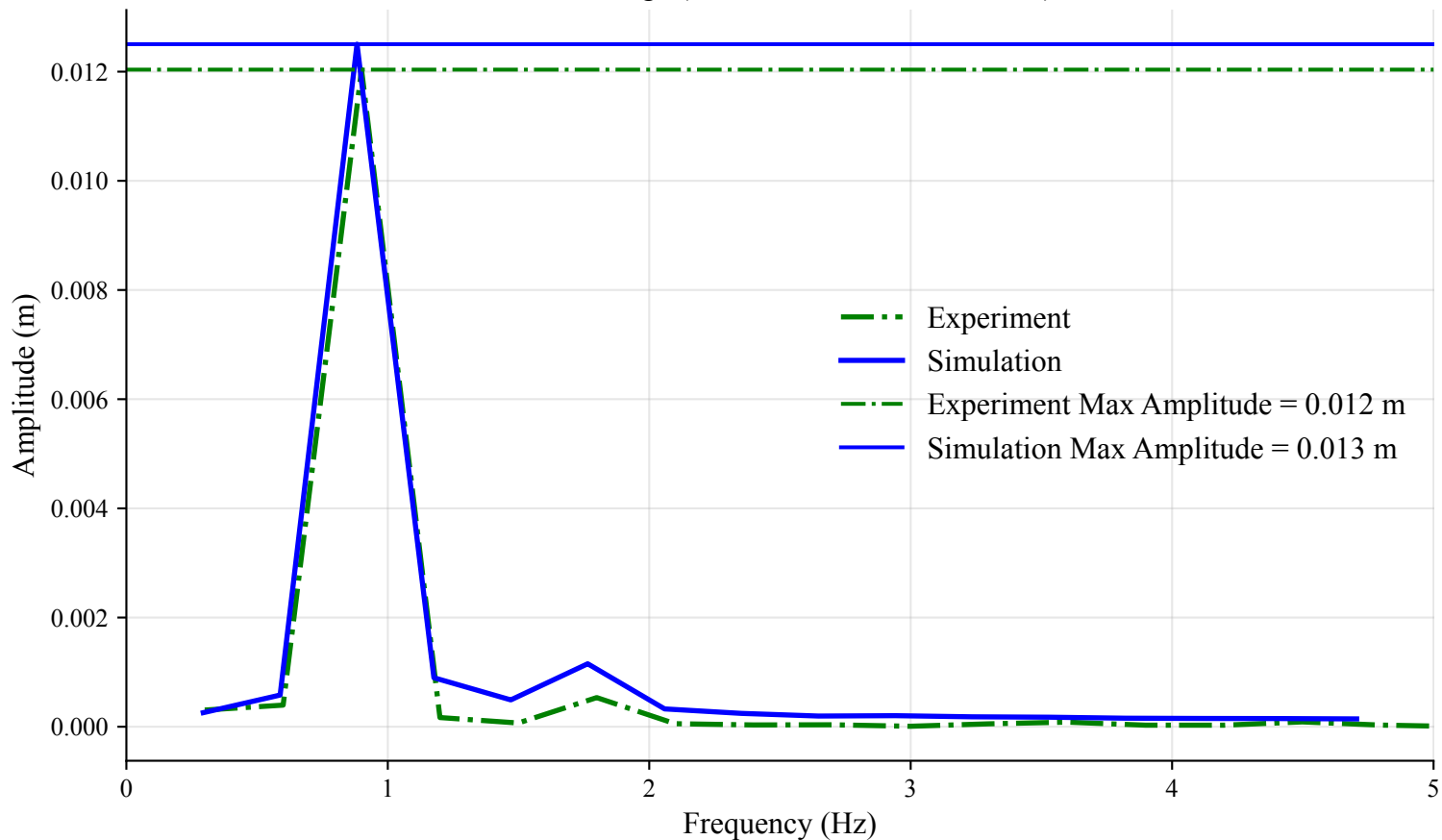
FFT of Surge (Time Window: 18s to 21.33s)
