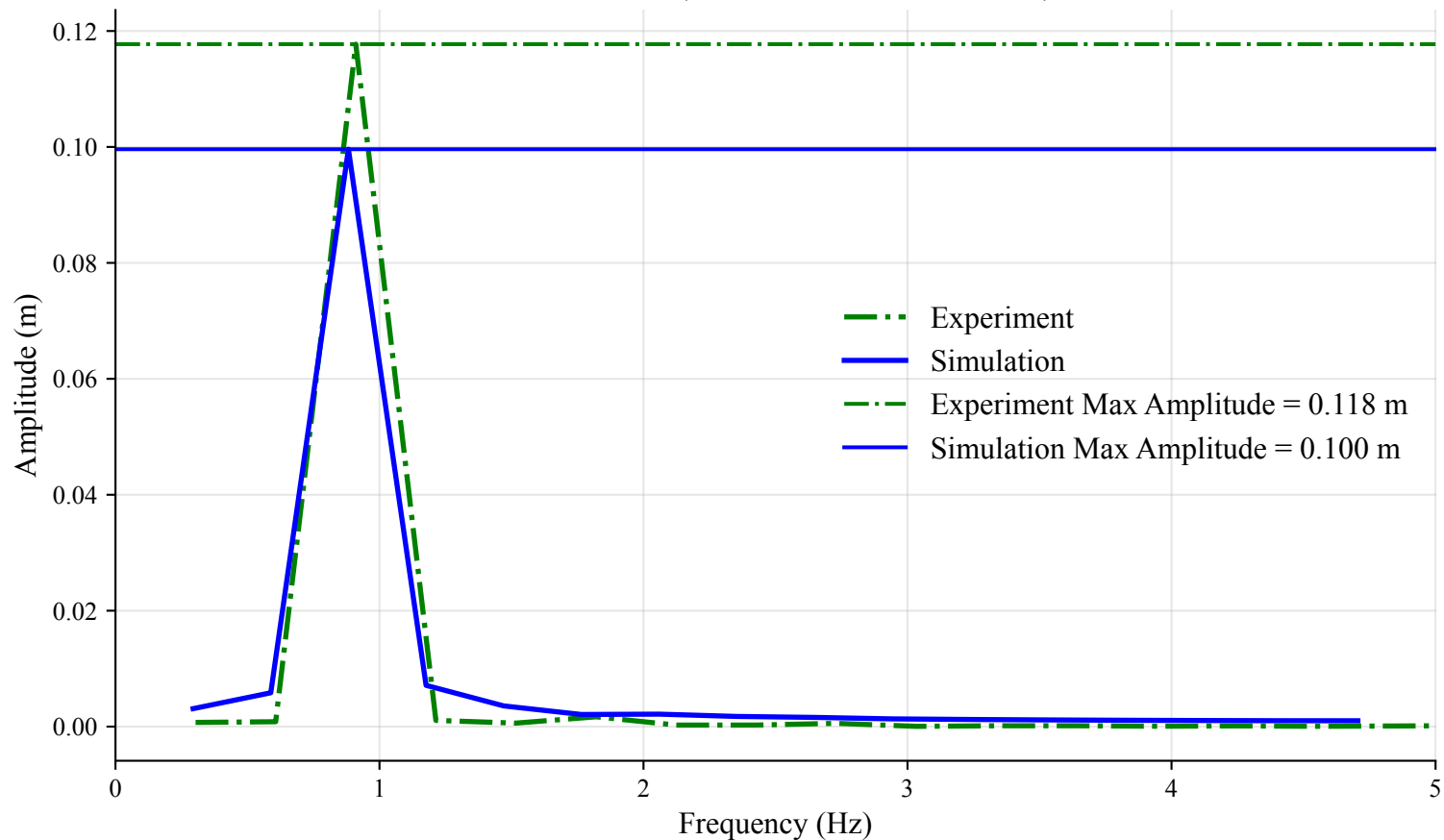
FFT of Heave (Time Window: 18s to 21.33s)
