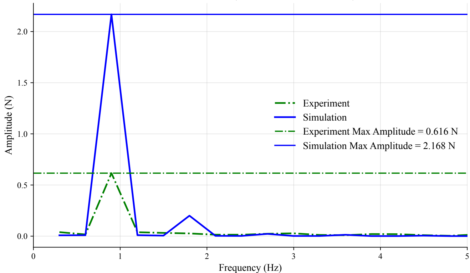
FFT of Front Tension (Time Window: 18s to 21.33s)
