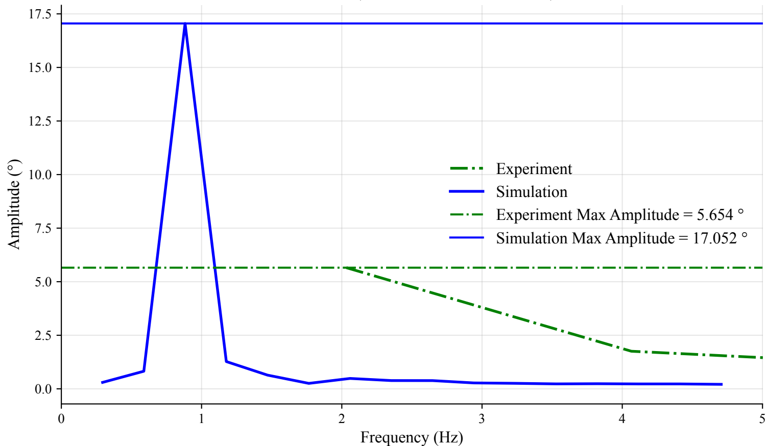
FFT of Pitch (Time Window: 18s to 21.33s)
