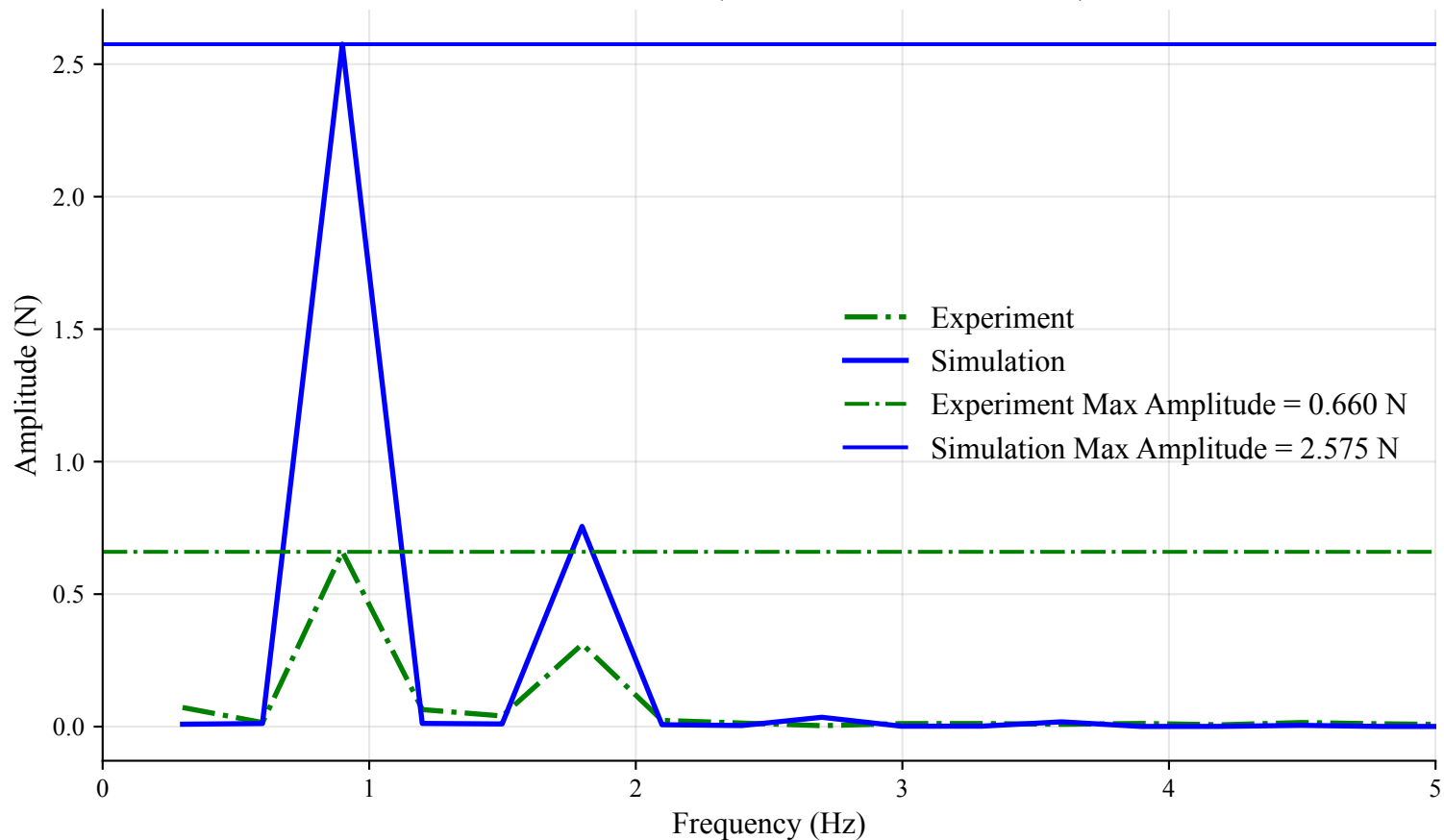
FFT of Rear Tension (Time Window: 18s to 21.33s)
