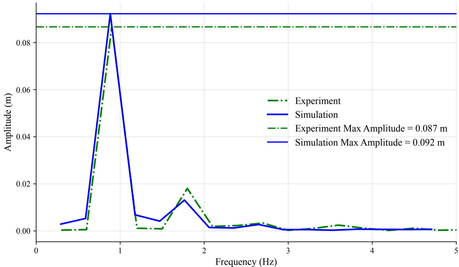
FFT of Wave Probe (Time Window: 18s to 21.33s)
