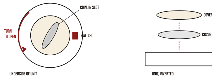
Fig. 5: The battery cover is opened with a coin. A nickel is ideal.
