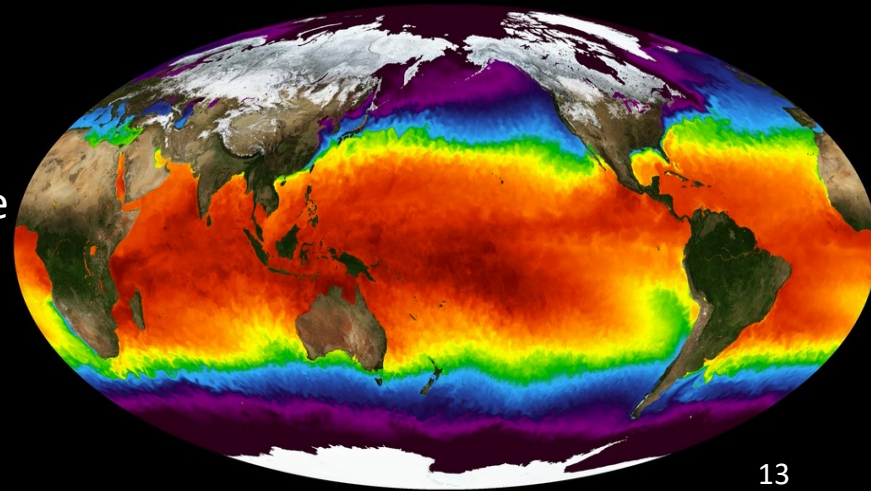
Satellite sea surface temperature (Earth surface temperature)
