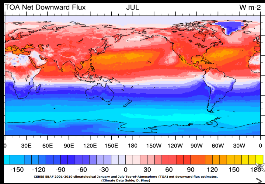
Top of atmosphere radiation (Energy fluxes)
