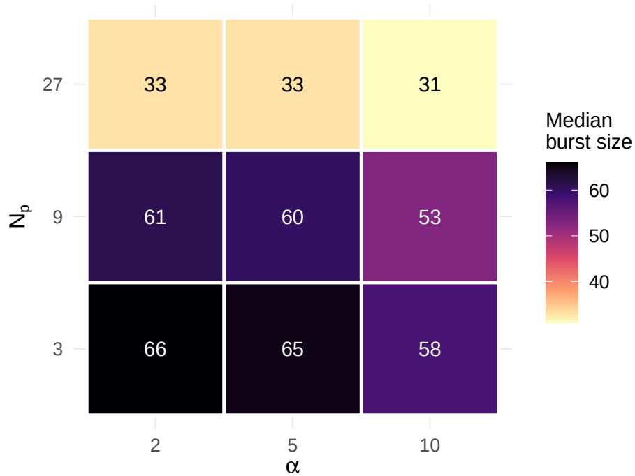
Median Burst Size
